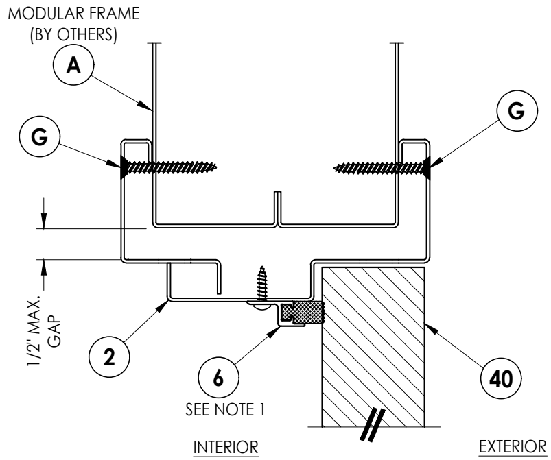
1 4 VERTICAL CROSS SECTION
