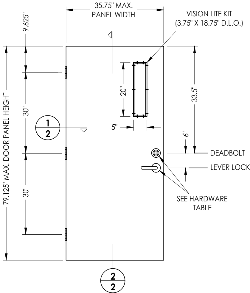
40 VISION HOLLOW METAL DOOR PANEL 6'-8" Door w/ Cylindrical Lock & Deadbolt
