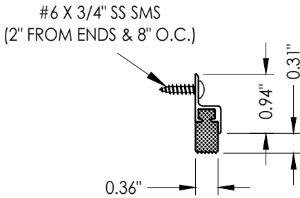
6 PERIMETER SEAL NGP 165 N-S
