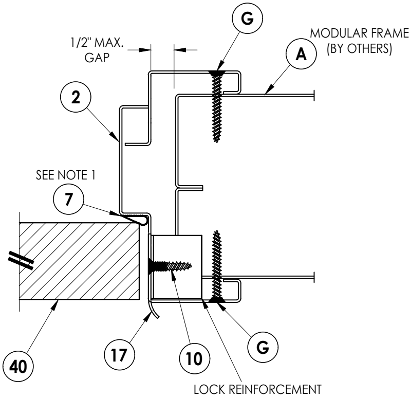
2 HORIZONTAL CROSS SECTION 3 Modular Frame Installation
