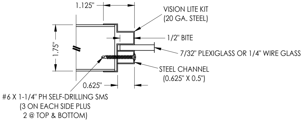
P1 VISION LITE KIT w/ PLEXIGLASS DETAIL
